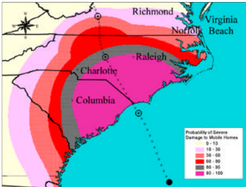
Use of CATS to determine the probability of structural damage to mobile homes on approach of Hurricane Fran. Image courtesy of SAIC
